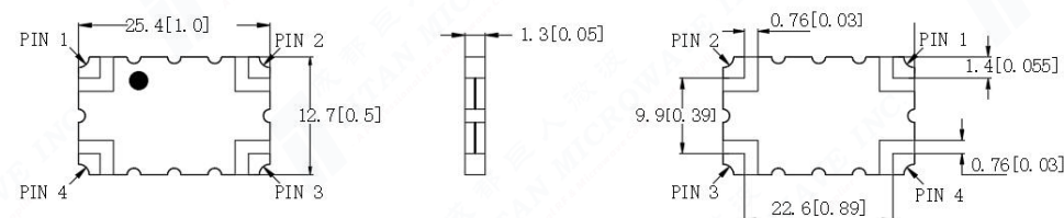
Top View
