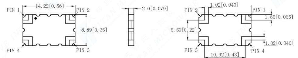
Top View
