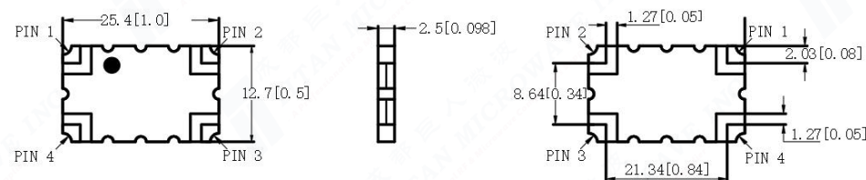
Top View
