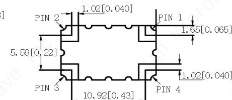
Bottom View
