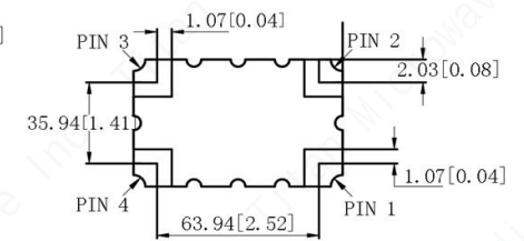
BOTTOM VIEW
